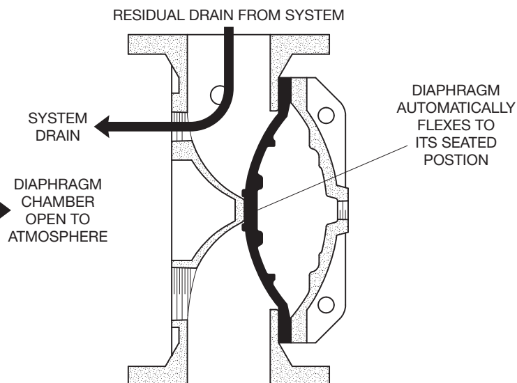
WATER SUPPLY SHUT OFF FIGURE 2D RESIDUAL DRAIN POSITION
