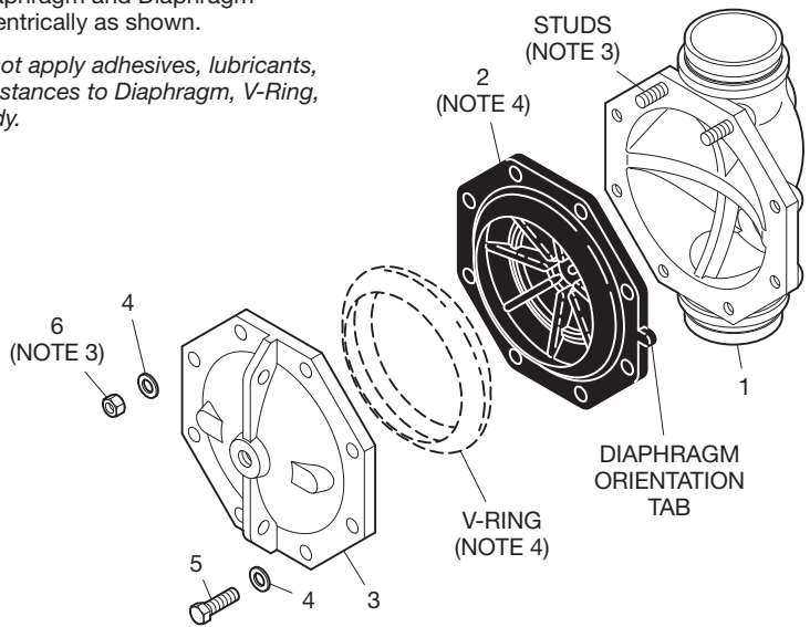
FIGURE 1 1-1/2 thru 8 INCH (DN40 thru DN200) DV-5 DELUGE VALVE ASSEMBLY
