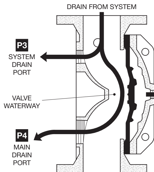
WATER SUPPLY SHUT OFF FIGURE 2C SYSTEM DRAIN POSITION
