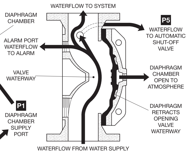
FIGURE 2B OPERATED POSITION
