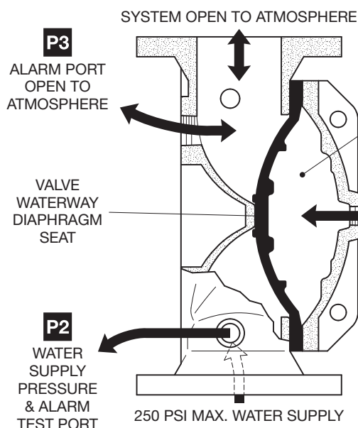
FIGURE 2A SET POSITION
