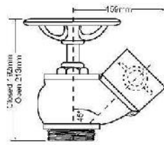
SCREW OBLIQUE LANDING VALVE
