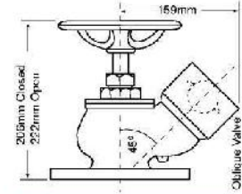
FLANGED OBLIQUE LANDING VALVE
