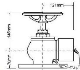
FLANGED RIGHT ANGLE VALVE
