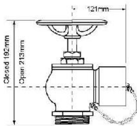
SCREW RIGHT ANGLE VALVE
